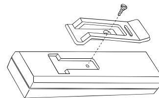
Figure 6. Belt Clip
