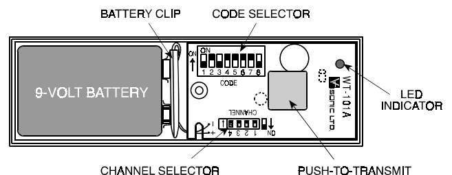
Figure 2. WT-101A, Cover Removed
