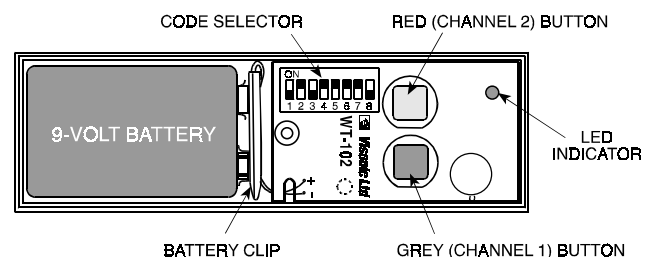
Figure 3. WT-102, Cover Removed
